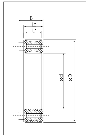
FenLock clamping elements type FLK 200 non self-centering
