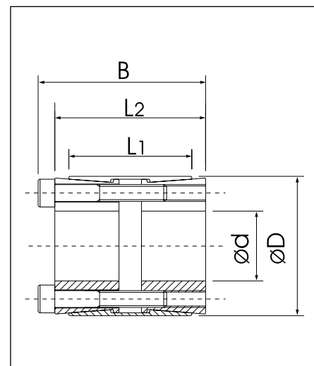
FenLock clamping elements type FLK 450 self-centering
